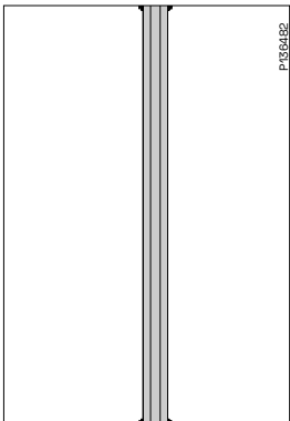
Pendant/Fixing rail 24/20FS can be mounted as a riser between the ceiling and floor using 4 Angle brackets 5L and 4 T-bolts.
