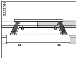
Join cable ladders to 90° bend using Joint 21.
