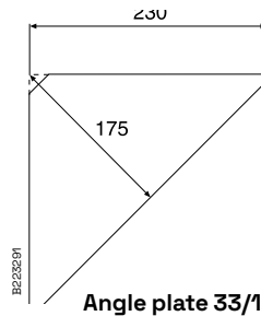
Angle plate 33/1
