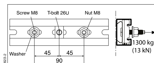
T-bolt 26U M10 + P/F-rail 24/48 + Washer 9x35x2
