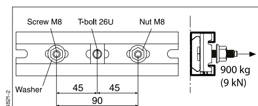
T-bolt 26U M8 + P/F-rail 24/48 + Washer 9x35x2
