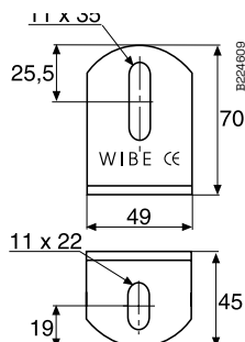
Angle bracket 5L
