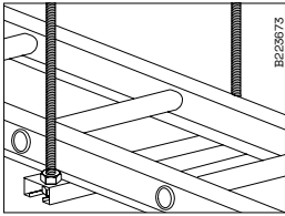
Support bracket HSO M10 installed with Threaded rod W76 M10.
