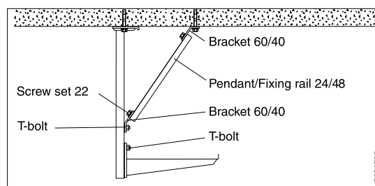
Use Bracket 60/40 together with Pendant/Fixing rail 24/48 to reduce the deflection of long Vertical pieces 2F, 20, 20F or 20FS. Cut the pendant/fixing rail to a suitable length on site.
