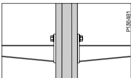
Mount Cantilever arm 50 using T-bolts.
