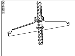
For installation of Support bracket 3 directly on ribbed bar 16-25 or fully threaded bar M16-M27.
