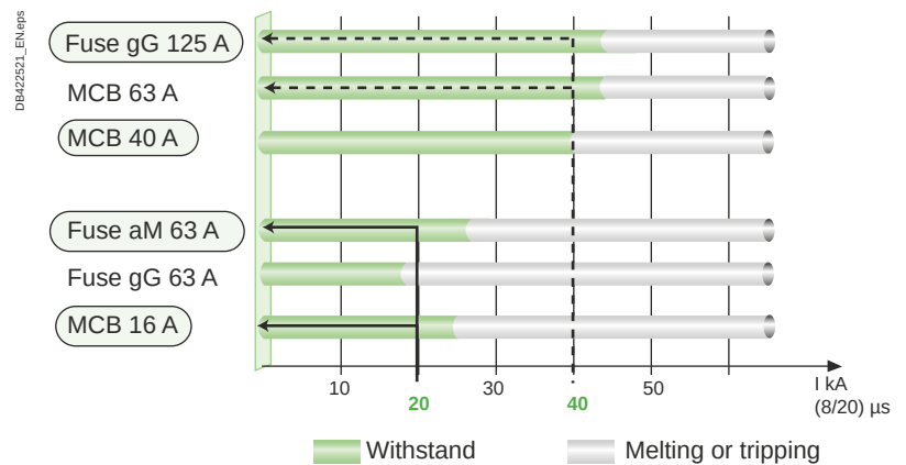
Fig. J56 Comparison of SCPDs voltage wave withstand capabilities for I_{max} = 20 kA and I_{max} = 40 kA
