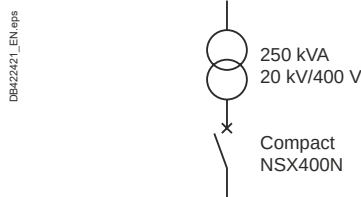
Fig. H43 Example of a transformer in a consumer's substation
