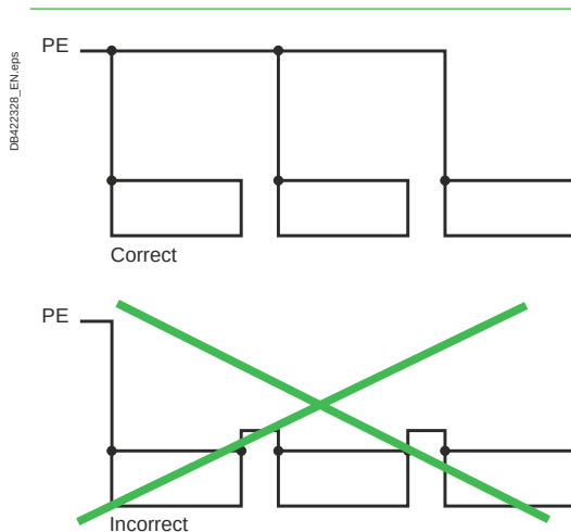
Fig. G55 A poor connection in a series arrangement will leave all downstream appliances unprotected
