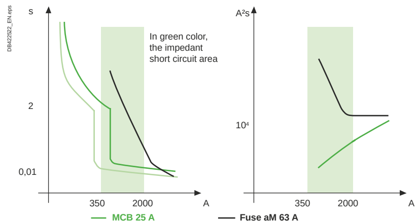
Fig. J57 Comparison of time/current and energy limitations curves for a circuit breaker and a fuse having the same 8/20 \mu s current wave withstand capability
