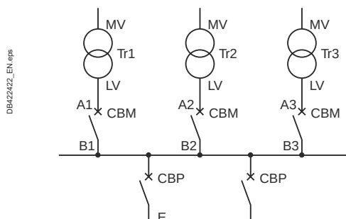
Fig. H44 Transformers in parallel
