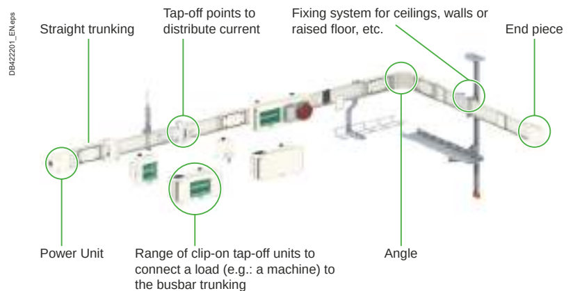
Fig. E44 Busbar trunking system design for distribution of currents from 25 to 4000 A
