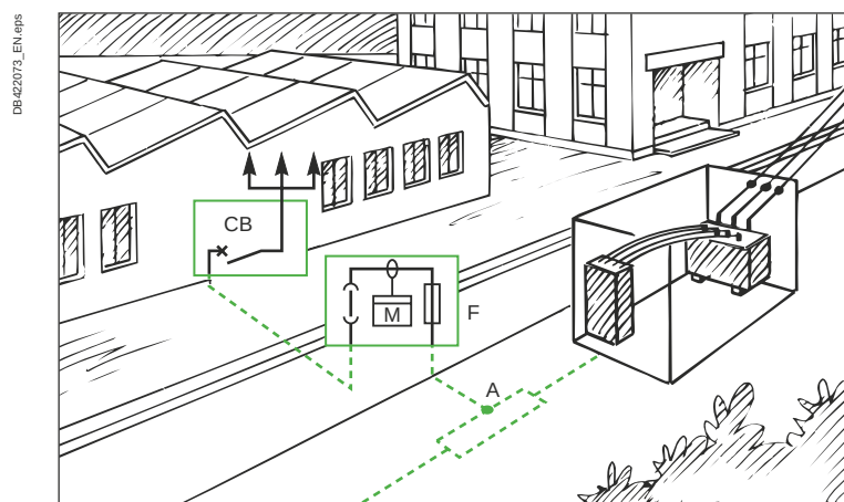
Fig. C6 Typical service arrangement for TT-earthed systems
