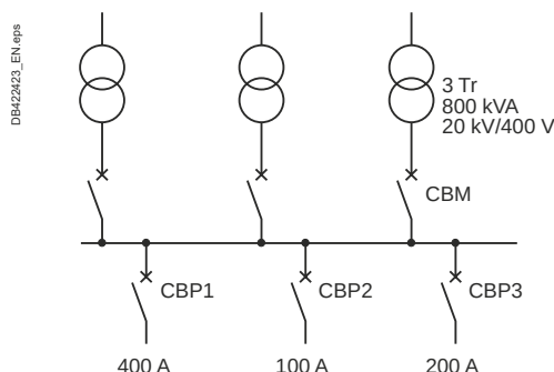
Fig. H45 Transformers in parallel
