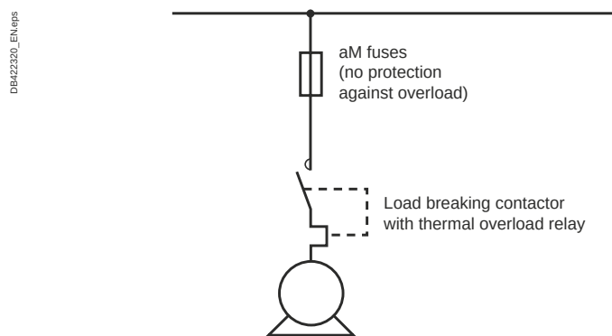
Fig. G43 Circuit protected by aM fuses
