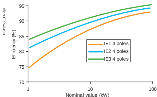
Fig. K16 Definition of energy efficiency classes for LV motors, according to Standard IEC60034-30
