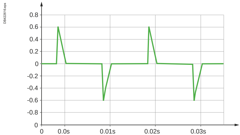
Fig. M7 Typical current waveform of a compact fluorescent lamp
