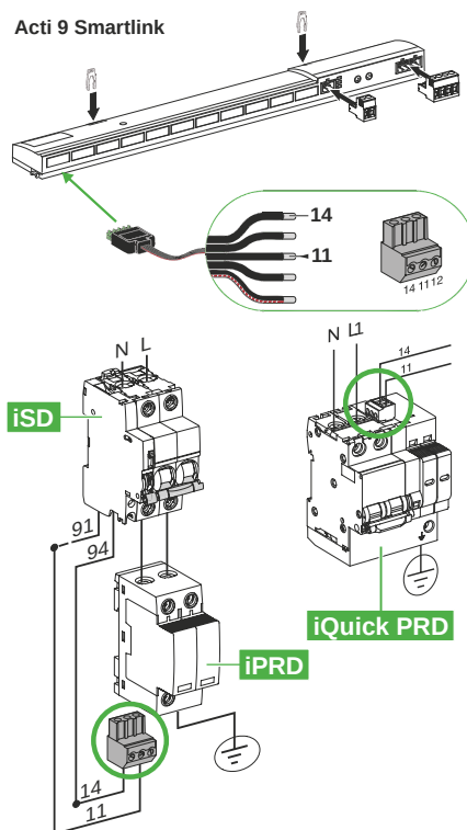
Fig. J55 Remote indication of SPD status using Smartlink
