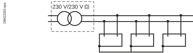
Fig. F68 Safety supply from a class II separation transformer
