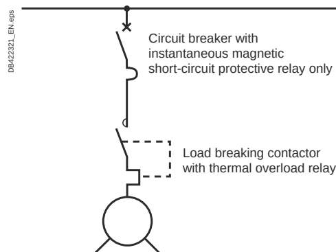
Fig. G44 Circuit protected by circuit breaker without thermal overload relay
