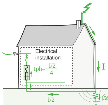
Fig. J30 Basic example of balanced impulse current distribution in 3 phase system
