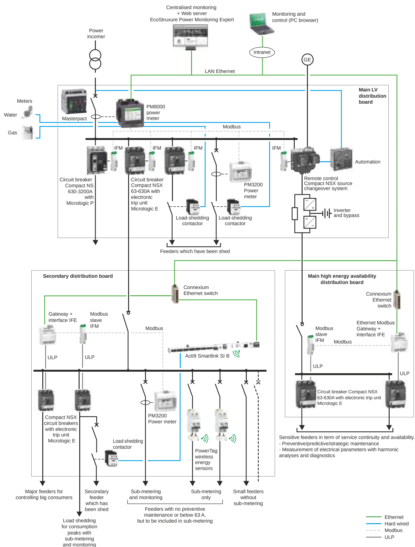
Fig. K31 Example of monitoring and control architecture for a large, sensitive industrial site
