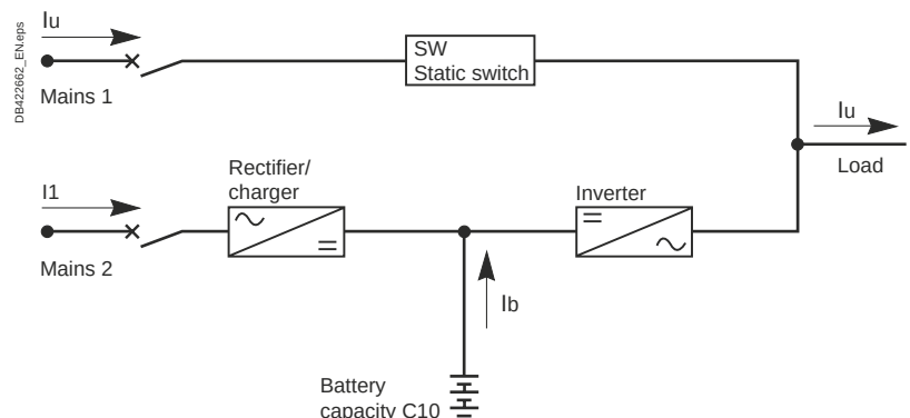
Fig. N28 Current to be taken into account for the selection of the wire connections
