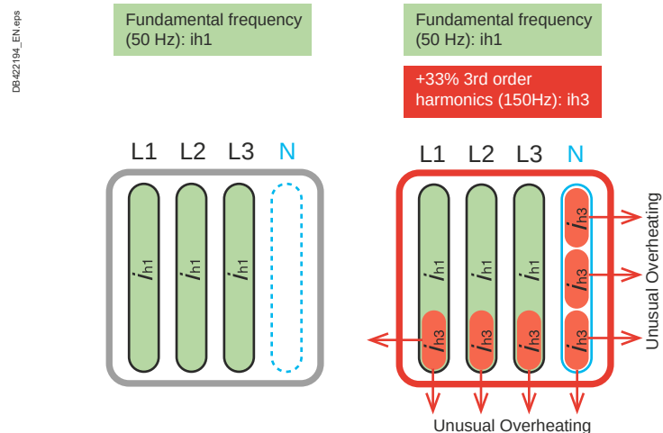
Fig. E59 Illustration of the overheating risk with standard busway sizing in presence of high level of 3rd harmonics
