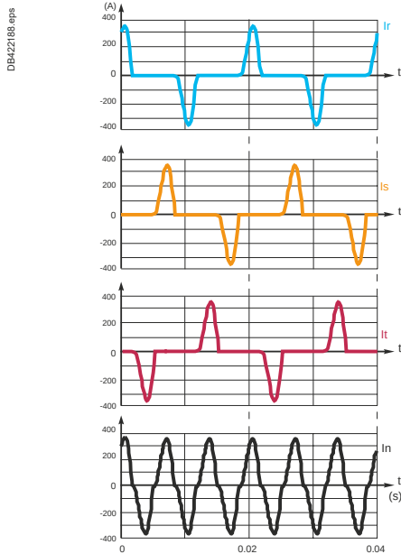
Fig. E52 Line and neutral currents absorbed by single-phase non-linear loads connected between phase and neutral.
